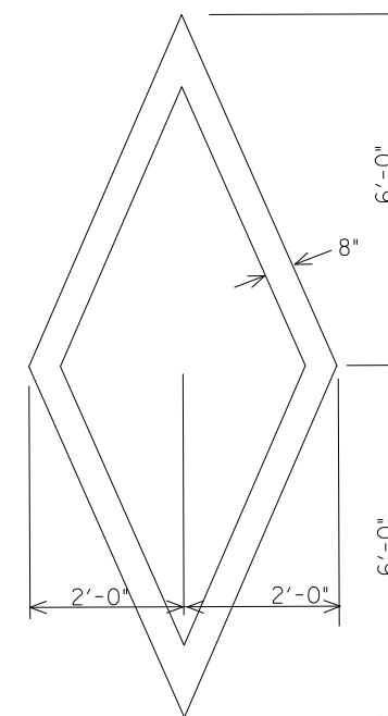
RESTRICTED LANE SYMBOL
