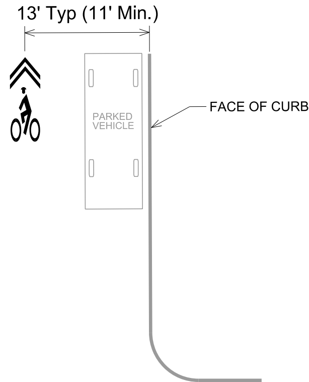
Sharrow Centerline WITH On Street Parking
