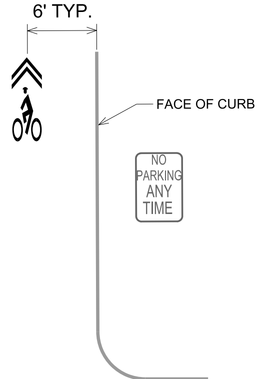
Sharrow Centerline NO On Street Parking
